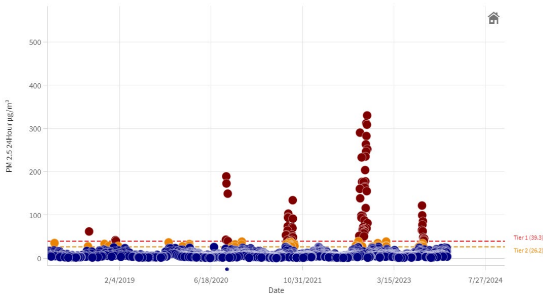
Figure 2: Time series plot of PM 2.5 daily combined site data for site 41-039-2013 (Oakridge, OR) 2018-2023. The tier thresholds are based on 2018-2022, the most recent 5-year period of certified data at the time of publication of this document. Tier 2 values are displayed as gold
