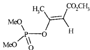
Alpha (cis) isomer
