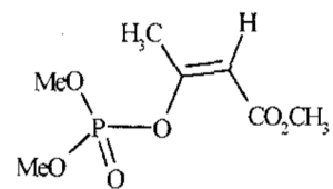
Beta (trans) isomer
