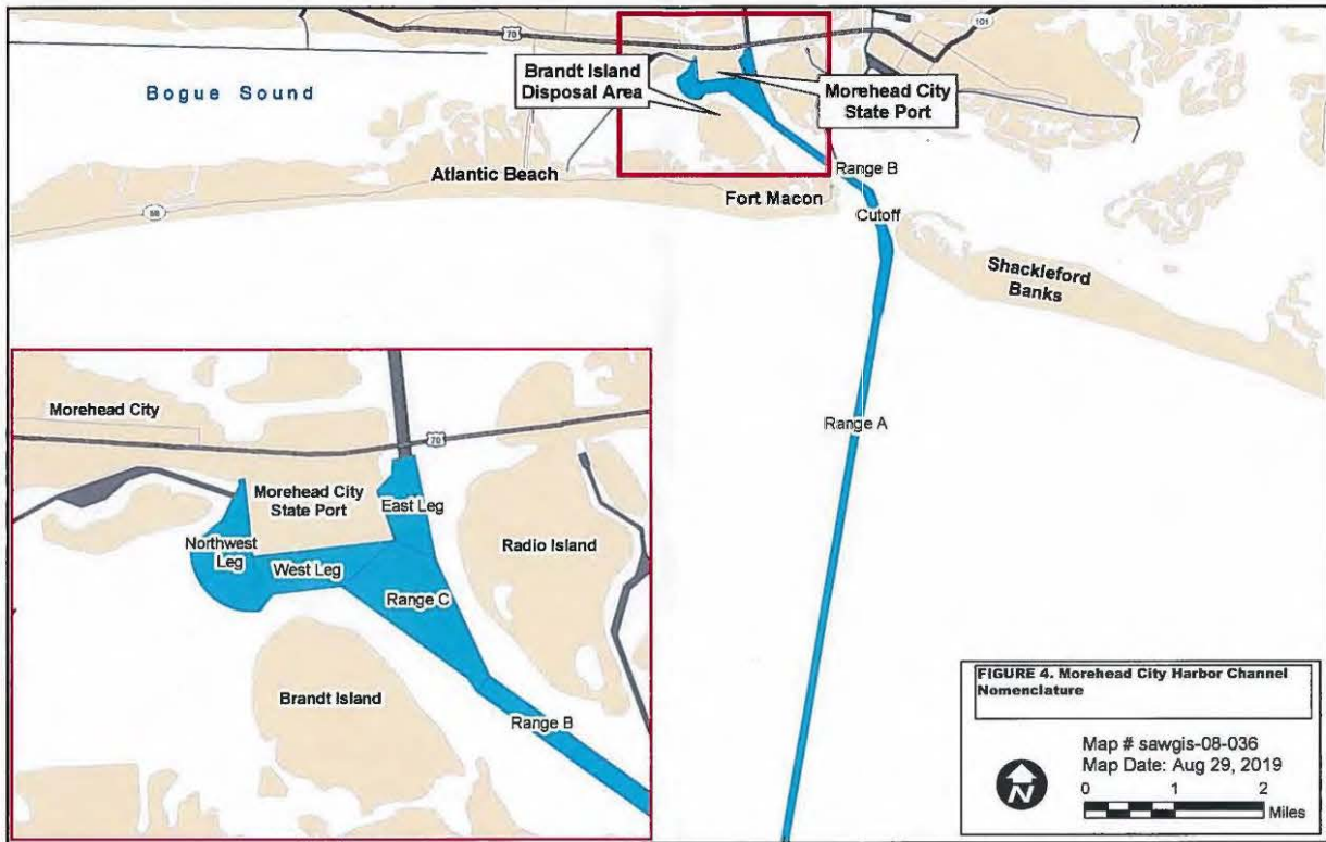
Figure 4. Morehead City Harbor Federal Navigation Project channel boundaries.
