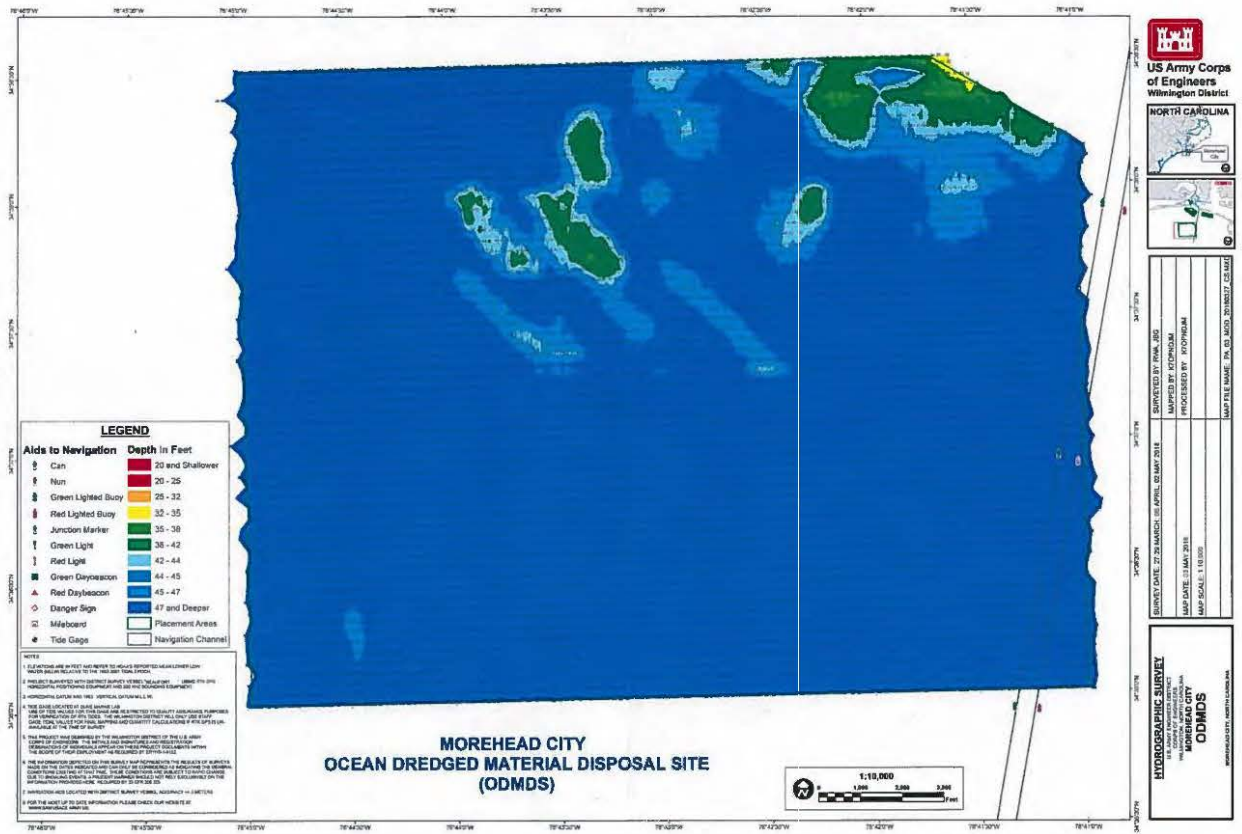
Figure 3. Morehead City Ocean Dredged Material Disposal Site Bathymetry (May 2018).
