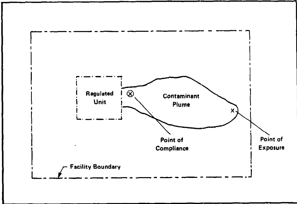
PLAN VIEW
