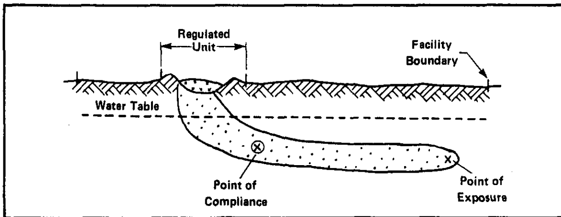
CROSS-SECTION VIEW
