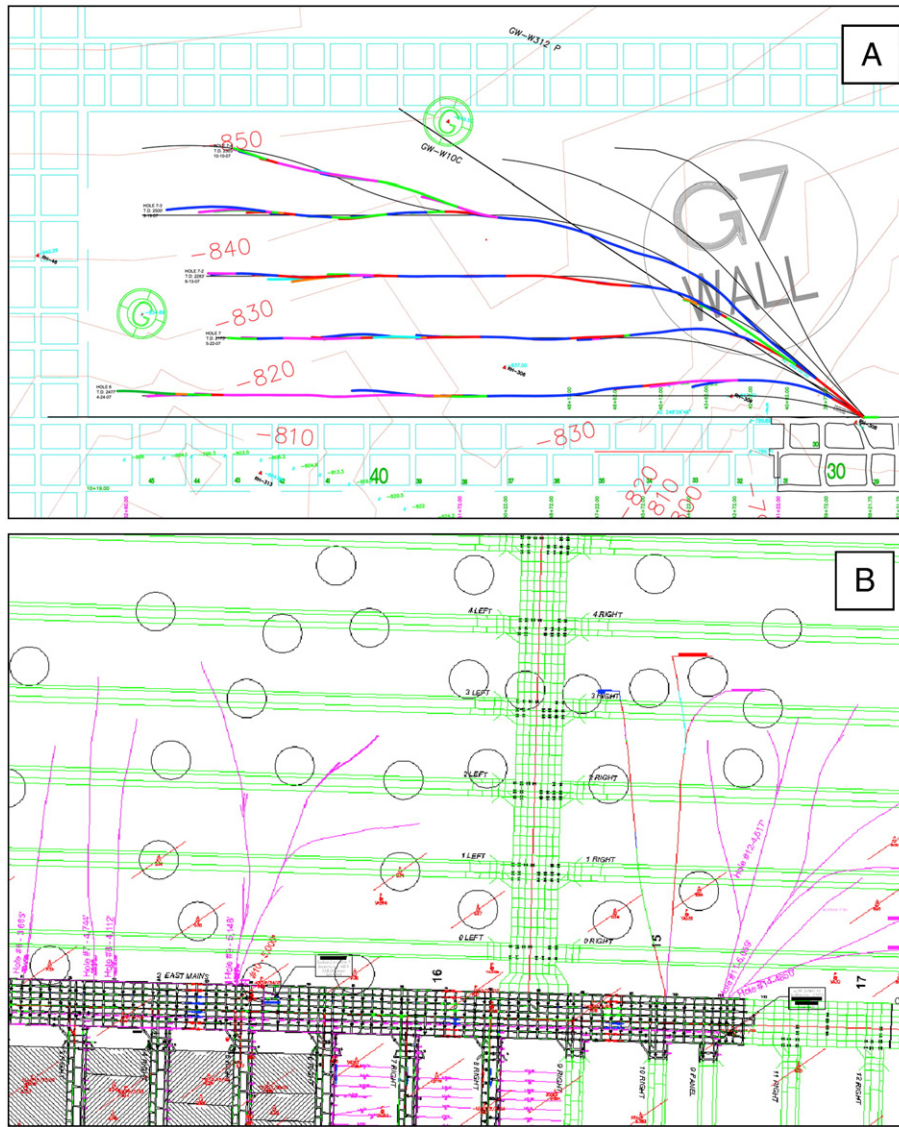
Fig. 6. Examples of using horizontal boreholes to reduce the in-place gas content of longwall panel (Bohan, 2009). Courtesy of REI Drilling.
