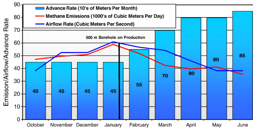
Fig. 4. Immediate impact of a 500-m shielding borehole along the gate road on emissions, advance rate, and ventilation air requirement (Bohan, 2009). Courtesy of REI Drilling.
